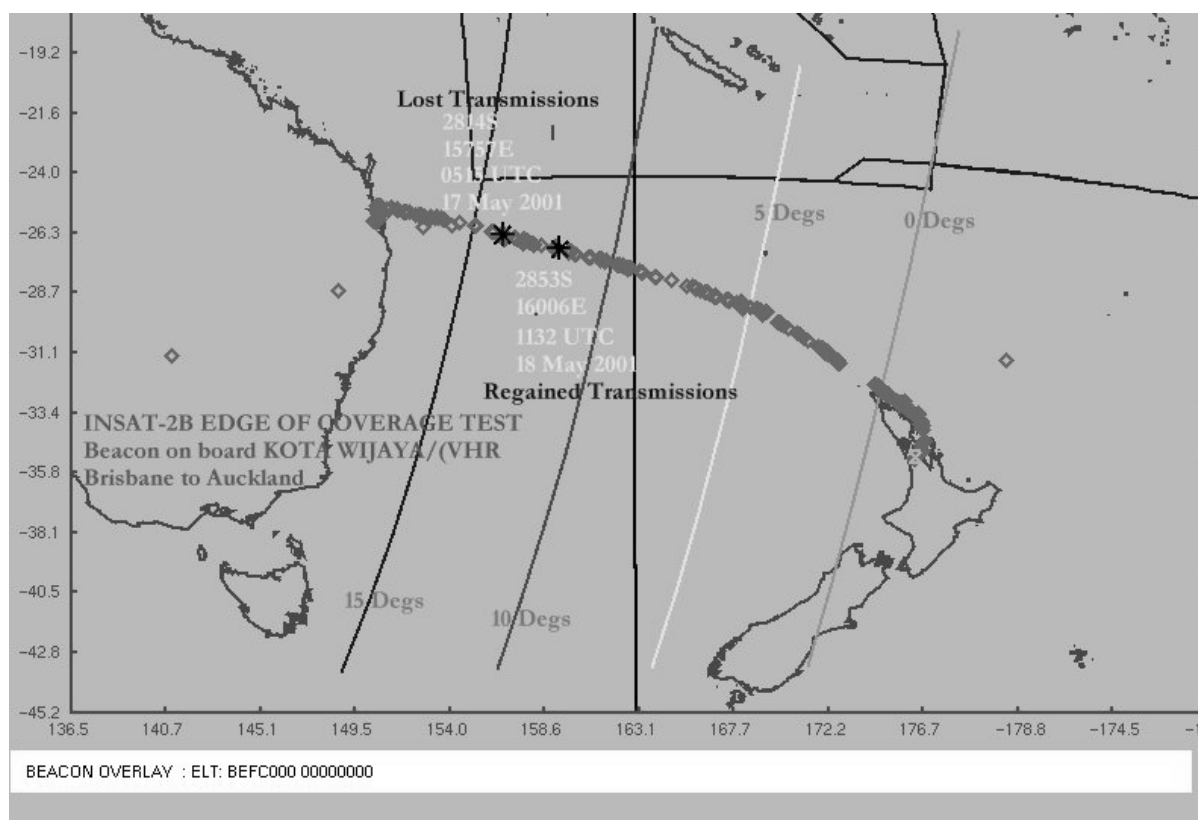
Figure 3-2: INSAT-2B, Loss of Beacon Detection at 0° Elevation
