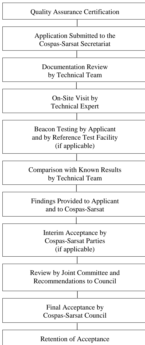
Figure 2.1: Process to Become a Cospas-Sarsat Accepted 406 MHz Beacon Type Approval Test Facility
