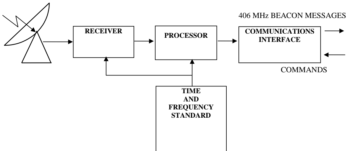
Figure 2.1: A Typical Cospas-Sarsat GEOLUT Functional Block Diagram
